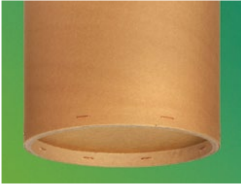
MDF bottom pressed against a tacked cardboard stop ring and jacket
